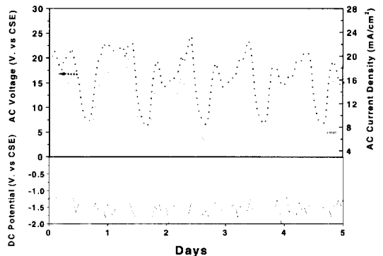
Fig. 3. An example of plot on measured AC voltage, corresponding AC current density and cathodic potential.
