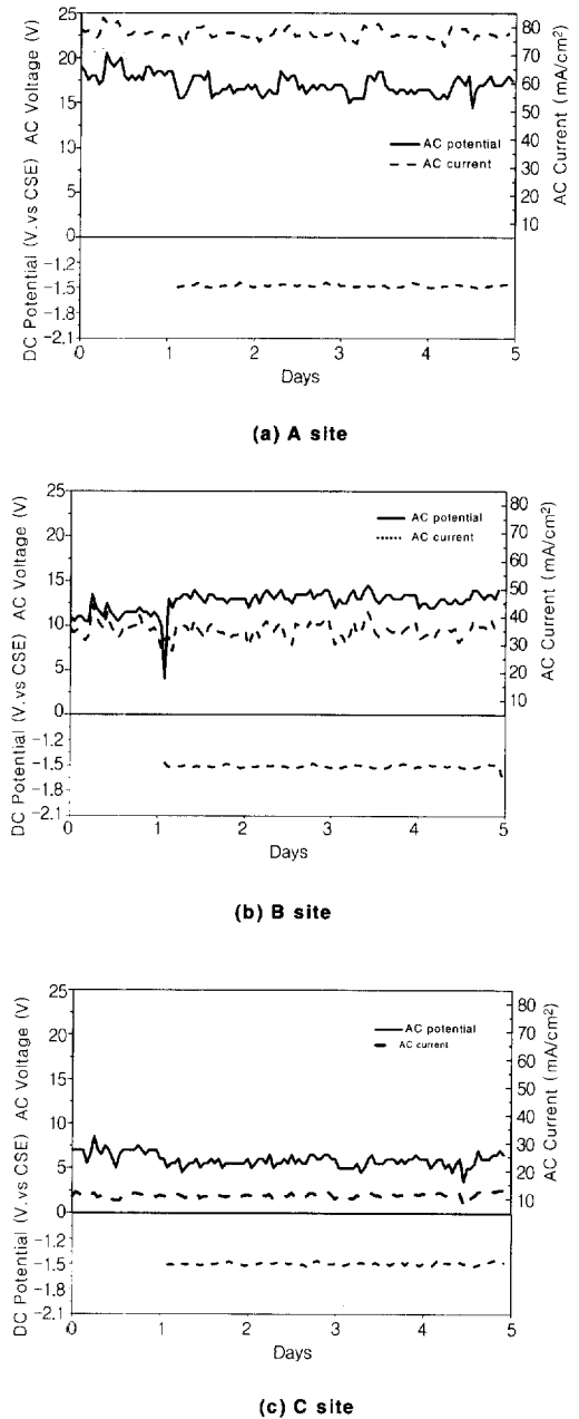
Fig. 9. Monitored results of AC voltage, AC current density and cathodic potential at CH1 place (A, B and C site is denoted position from AC interference source).
