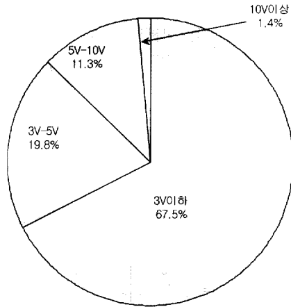
Fig. 1. Distribution of AC voltages measured in 3,823 test boxes.
