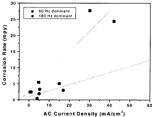
Fig. 5. Dependence of corrosion rate on AC frequency.
