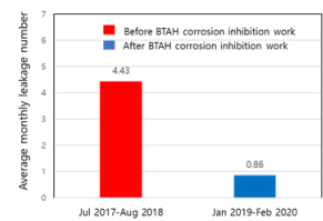
Fig. 11 Average monthly leakage number before and after BTAH corrosion inhibition work.
