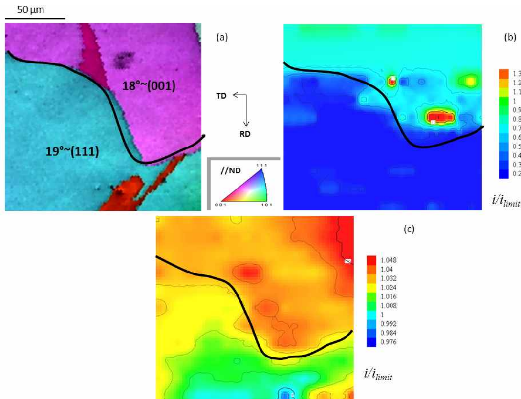
Fig. 3 Combined inverse pole figure (IPF)/image quality (IQ) map (a) and corresponding SECM current map after passivation at E = 0.1 \text{ V} during 30min (b) corresponding SECM current map after the cathodic reduction of the passive layer (c). Measurements in sodium hydrogen orthophosphate/sodium hydroxide buffer solution containing 5mM ferrocenemethanol. Scanned area 200 \mu\text{m} in x and y direction with dx=10 \mu\text{m} and dy=20 \mu\text{m} [2].
