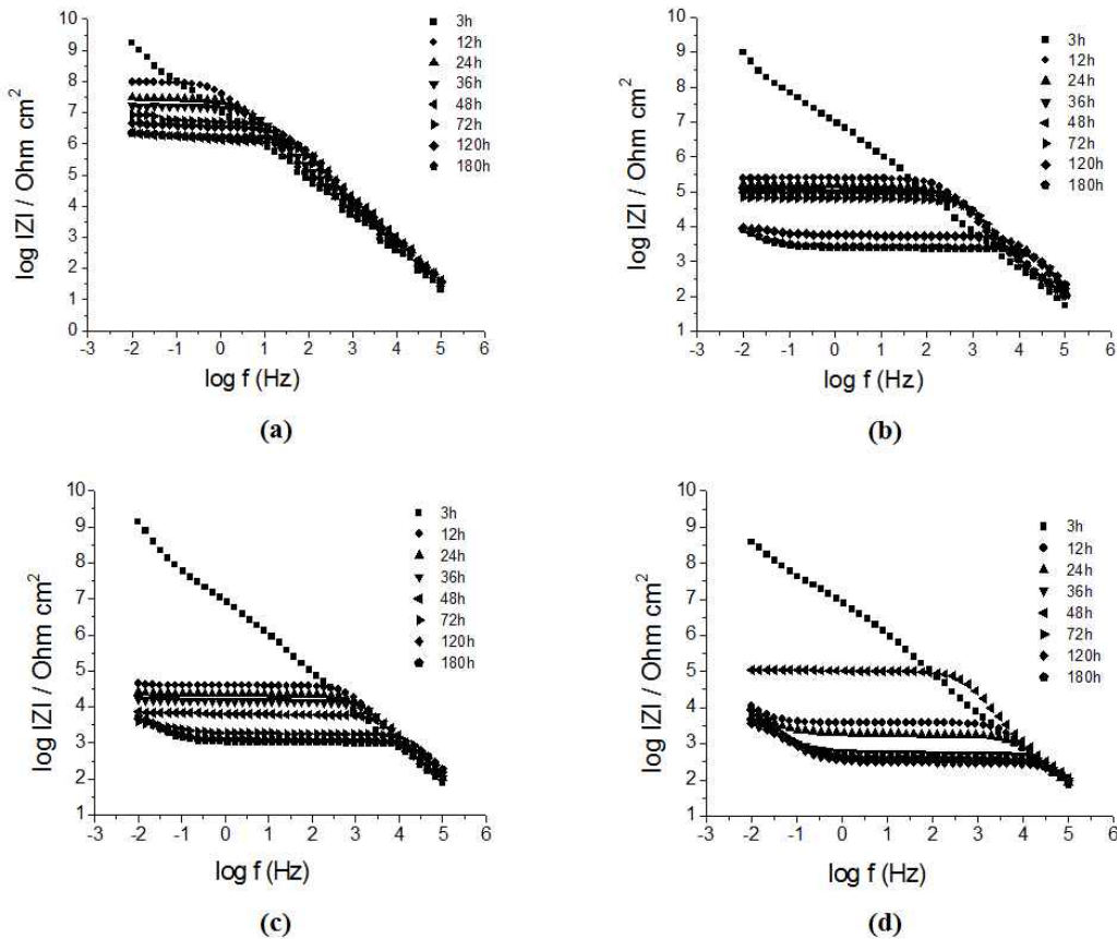
Fig. 6. EIS spectra in Bode plot for polyester-melamine coatings with various contents of natural wood fiber as a function of immersion time: (a) pure (b) 5 wt% of NWF; (c) 10 wt% of NWF; and (d) 20 wt%. of NWF.
